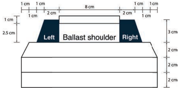
Dimension of Railway track
